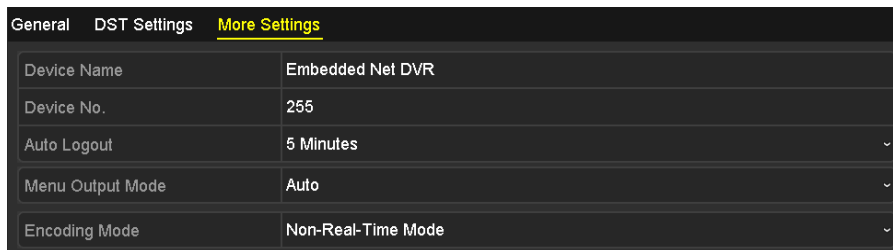
Figure 5-49 More Settings
