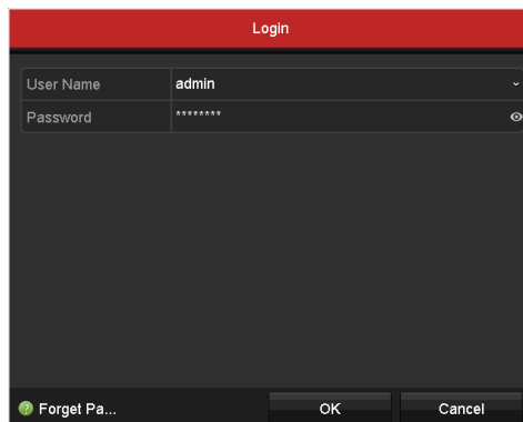
Figure 2-28 Login Interface
