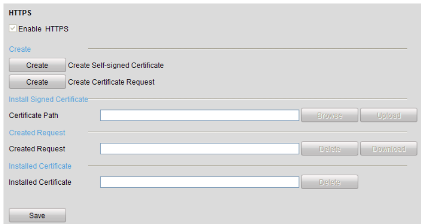
Figure 12-19 HTTPS Settings
