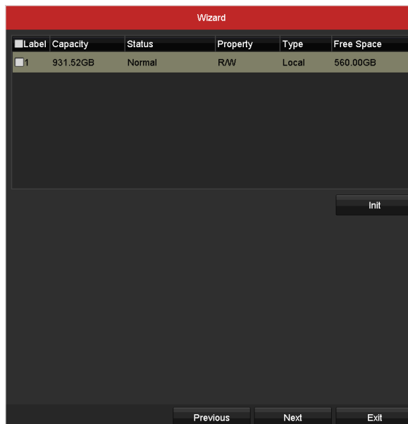
Figure 2-25 HDD Management
