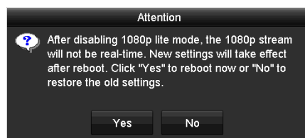
Figure 5-46 Attention
