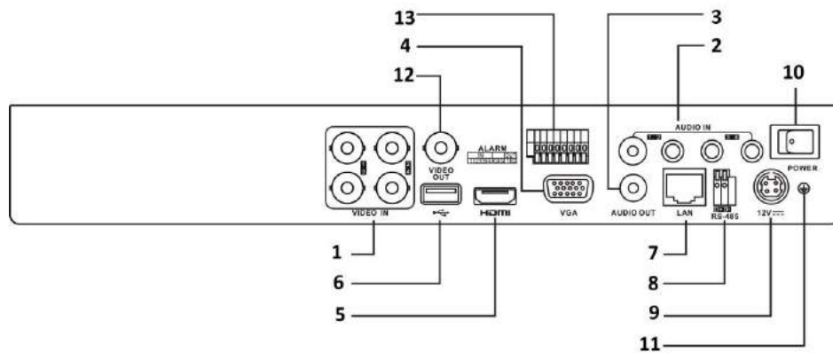
Figure 1-16 Rear Panel of DS-7200HUHI-F/N and 7600HUHI-F/N
