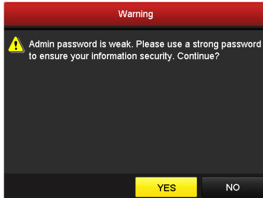
Figure 2-4 Warning
